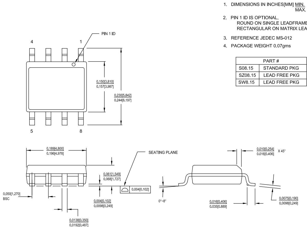
Figure 20. 8-pin SOIC (150 Mils) Package Outline, 51-85066
