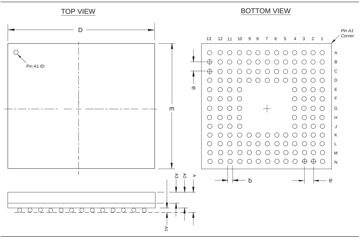
Figure 7-6. 144-Pin Micro FineLine BGA Package Outline
