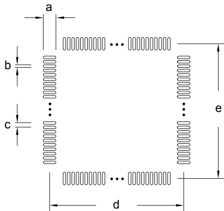
Figure 7.4. LQFP100 PCB Stencil Design
