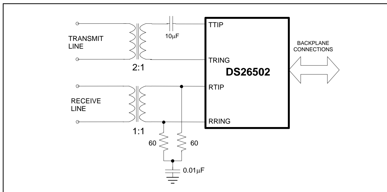
Figure 13-1. Basic Network Connection
