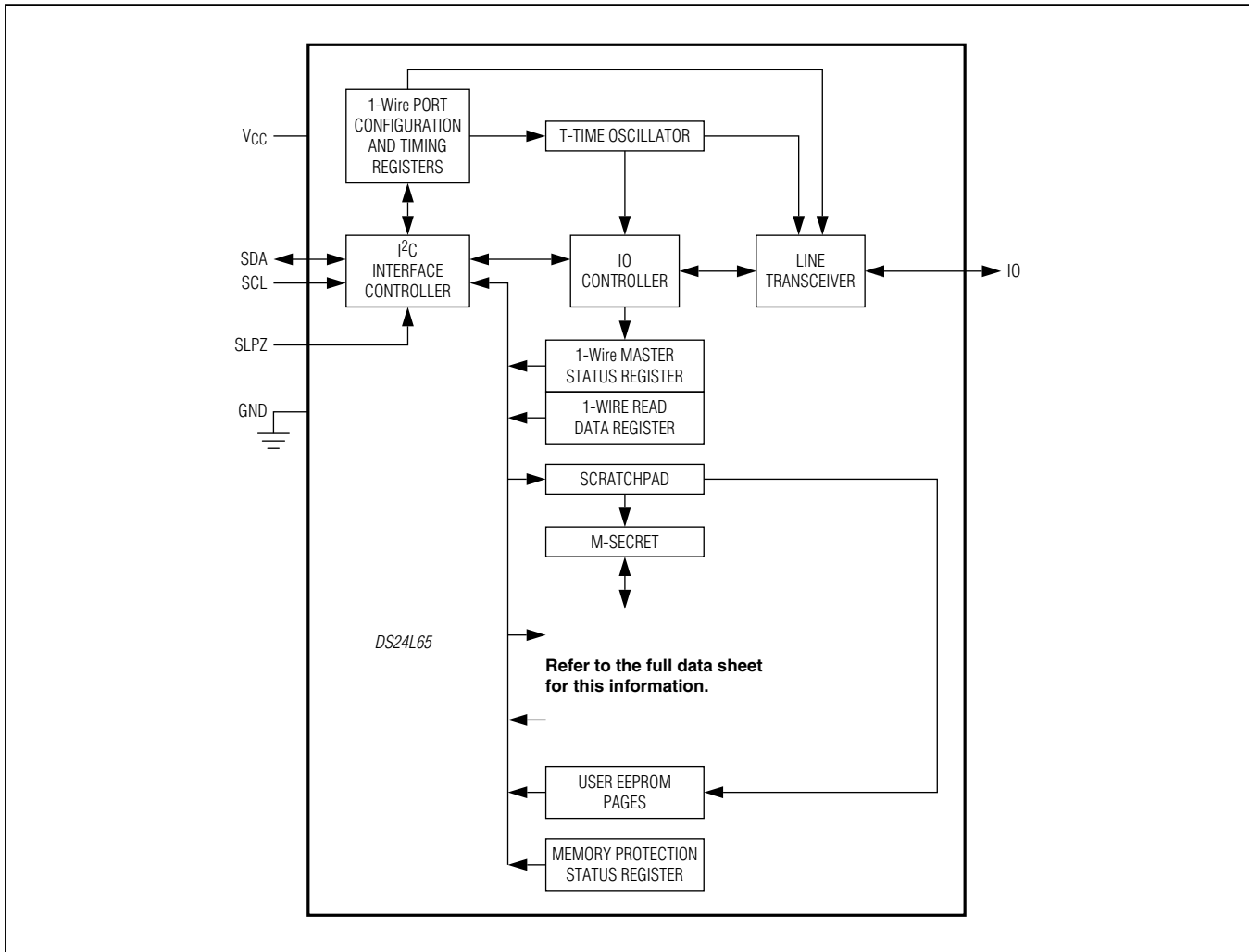
Figure 1. Block Diagram
