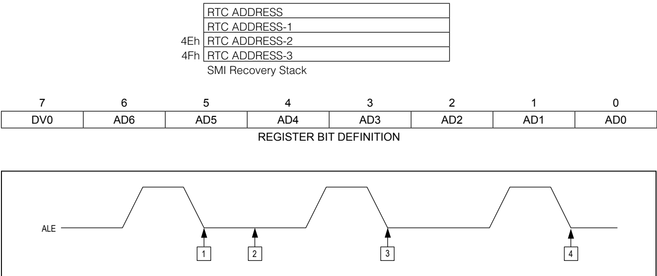
Figure 8. ALE Waveform
