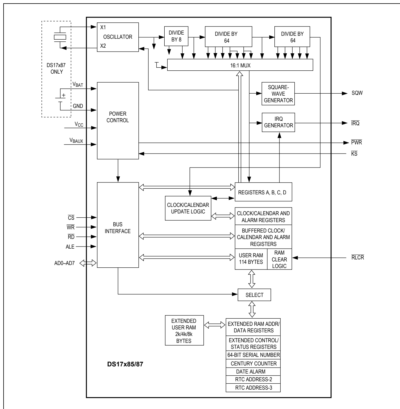
Figure 1. Functional Diagram
