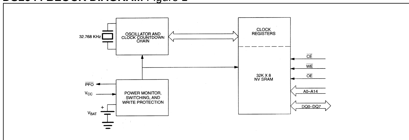
DS1644 BLOCK DIAGRAM Figure 1
