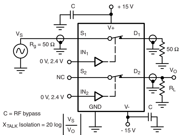
Figure 4. Channel-to-Channel Crosstalk
