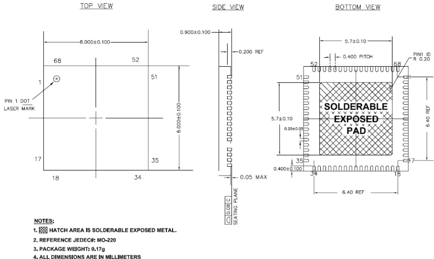
Figure 9. 68-Pin ( 8 \times 8 \times 0.90 mm) QFN (Sawn Type)
