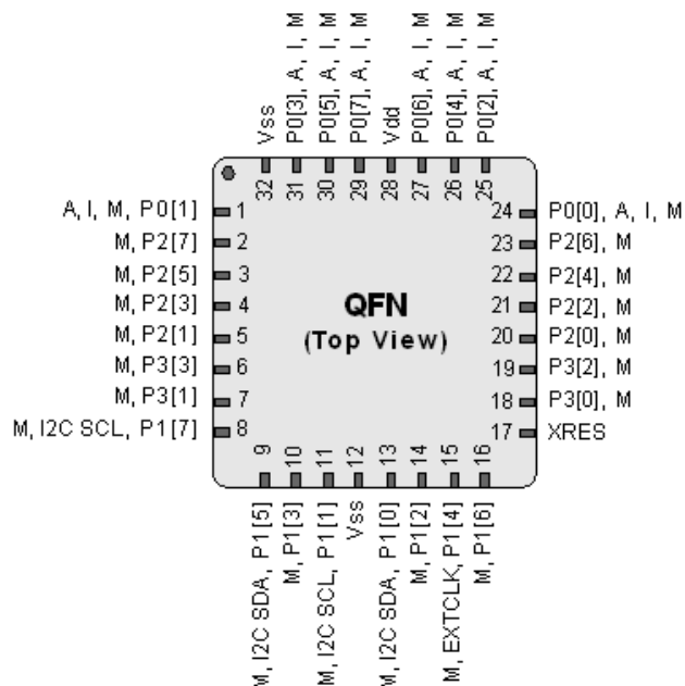
Figure 9. CY8C21434B 32-pin Sawn PSoC Device Sawn
