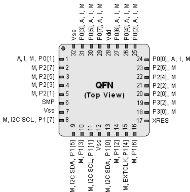
Figure 10. CY8C21634B 32-pin Sawn PSoC Device Sawn
