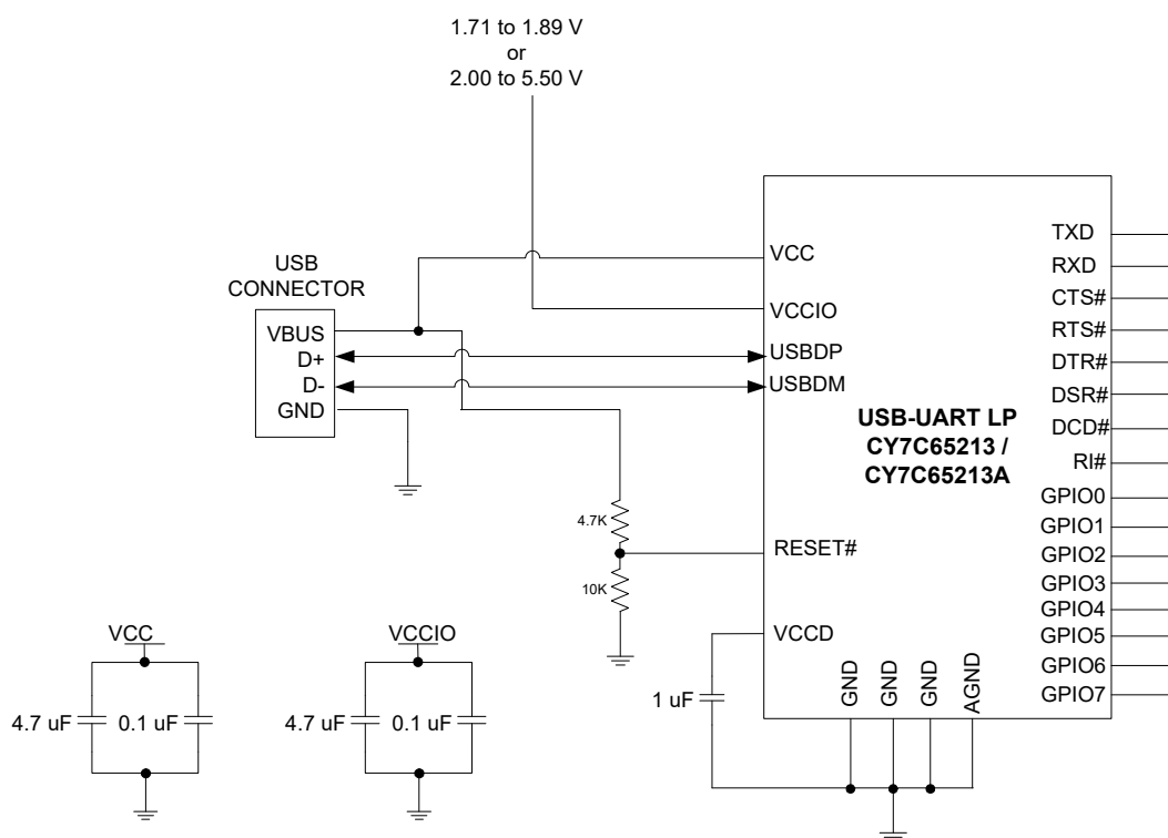
Figure 2. Self-Powered Configuration
