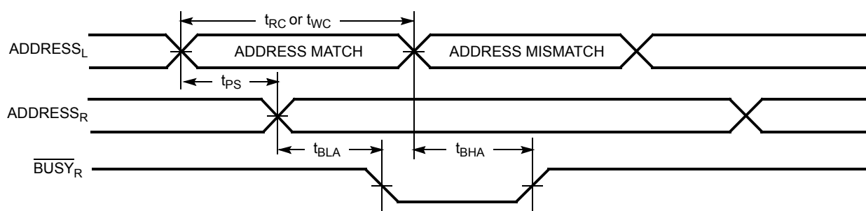
Figure 13. Busy Timing Diagram No. 2 (Address Arbitration) [35]
