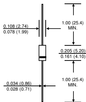
DO-41
