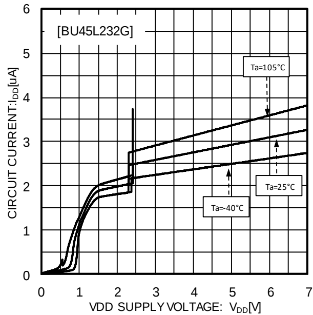
Fig.3 Circuit Current
