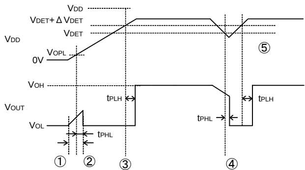
Fig.15 Timing Waveform
