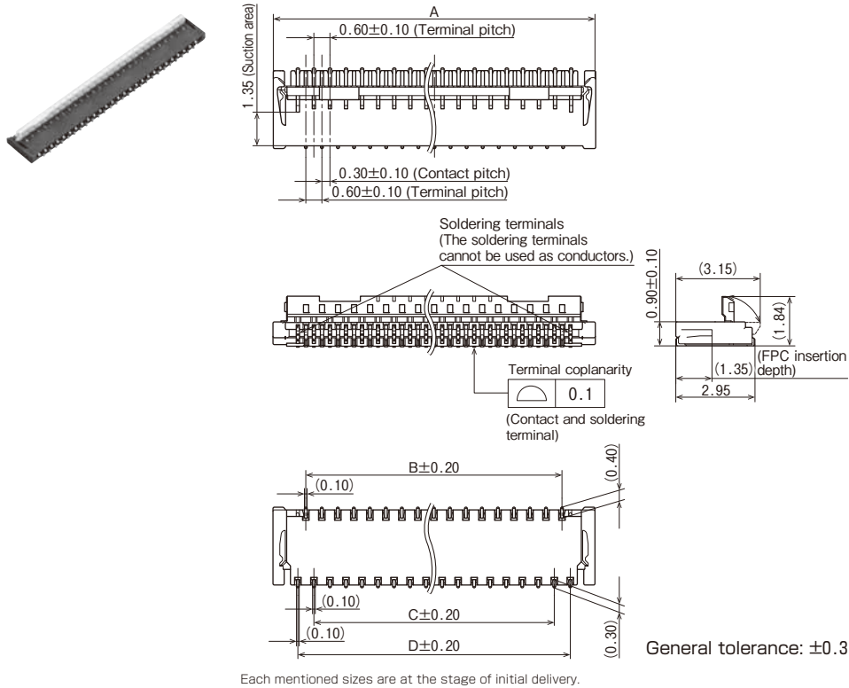
Dimension table
