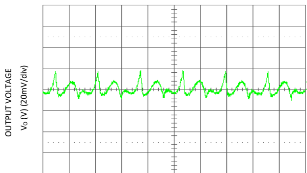
Figure 8. Typical Output Ripple and Noise ( V_{in} = 12.0Vdc , V_o = 2.5Vdc , I_o = 10A ).
