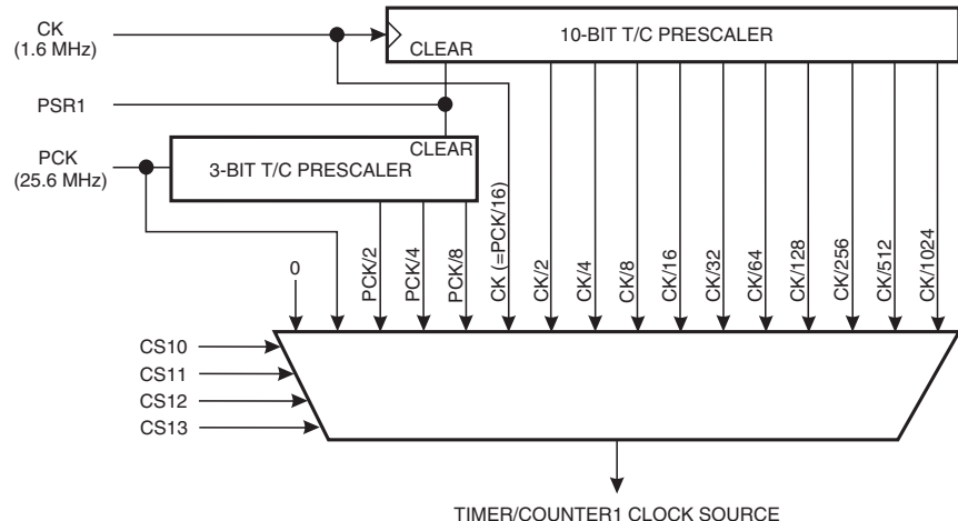
Figure 19. Timer/Counter1 Prescaler
