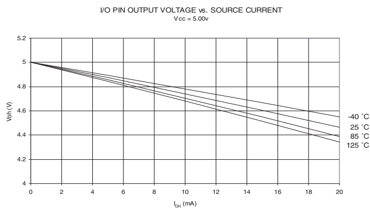
Figure 28-13. Output High Voltage vs. Output High Current ( V_{CC} = 5.0V )
