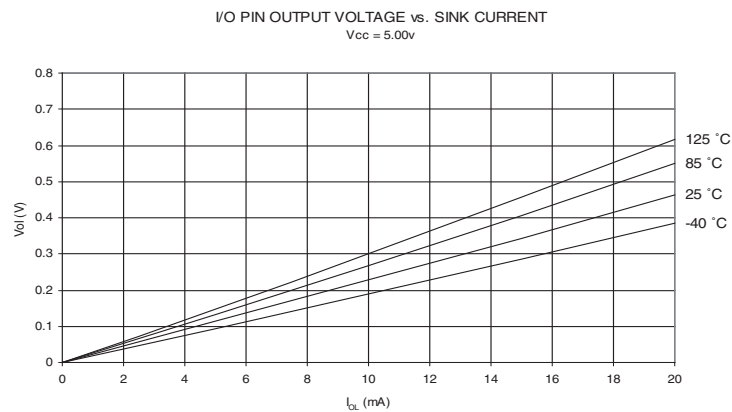
Figure 28-6. Output Low Voltage vs. Output Low Current ( V_{CC} = 5V )
