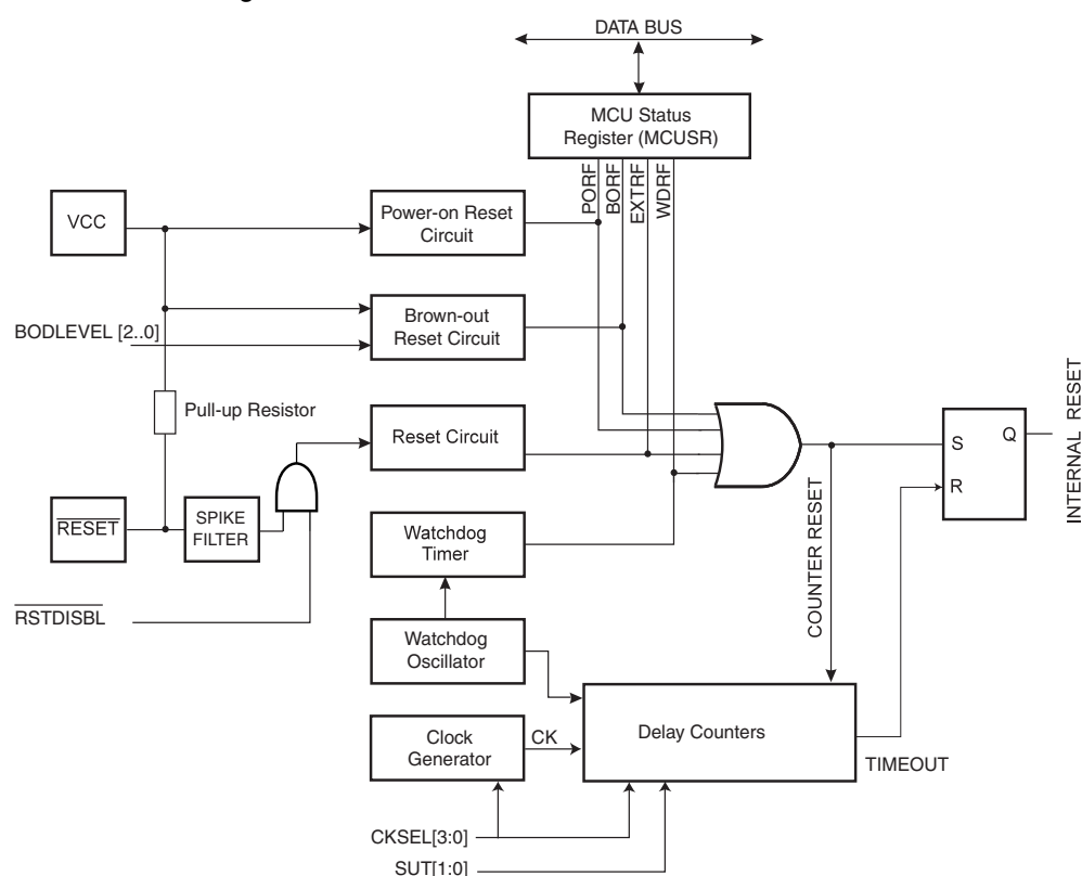
Figure 8-1. Reset Logic
