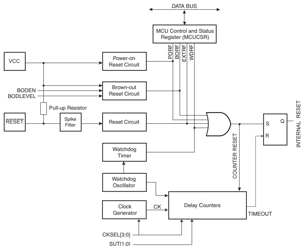
Figure 22. Reset Logic
