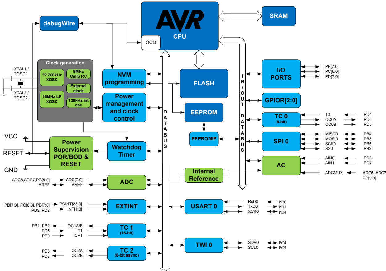
Figure 4-1. Block Diagram
