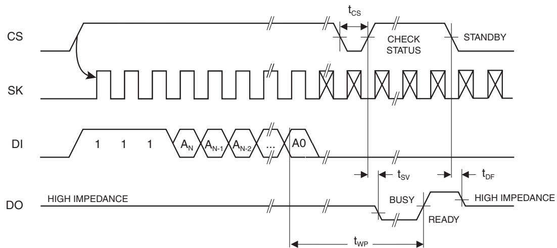
Figure 5-7. ERASE Timing
