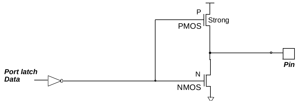
Figure 25. Push-pull Output
