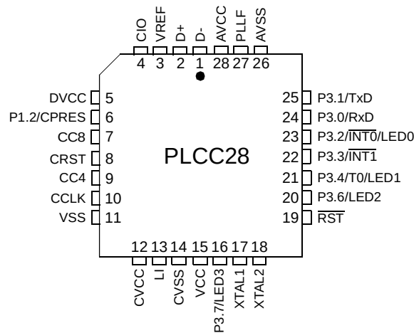
Figure 6. PLCC28 Package Pinout
