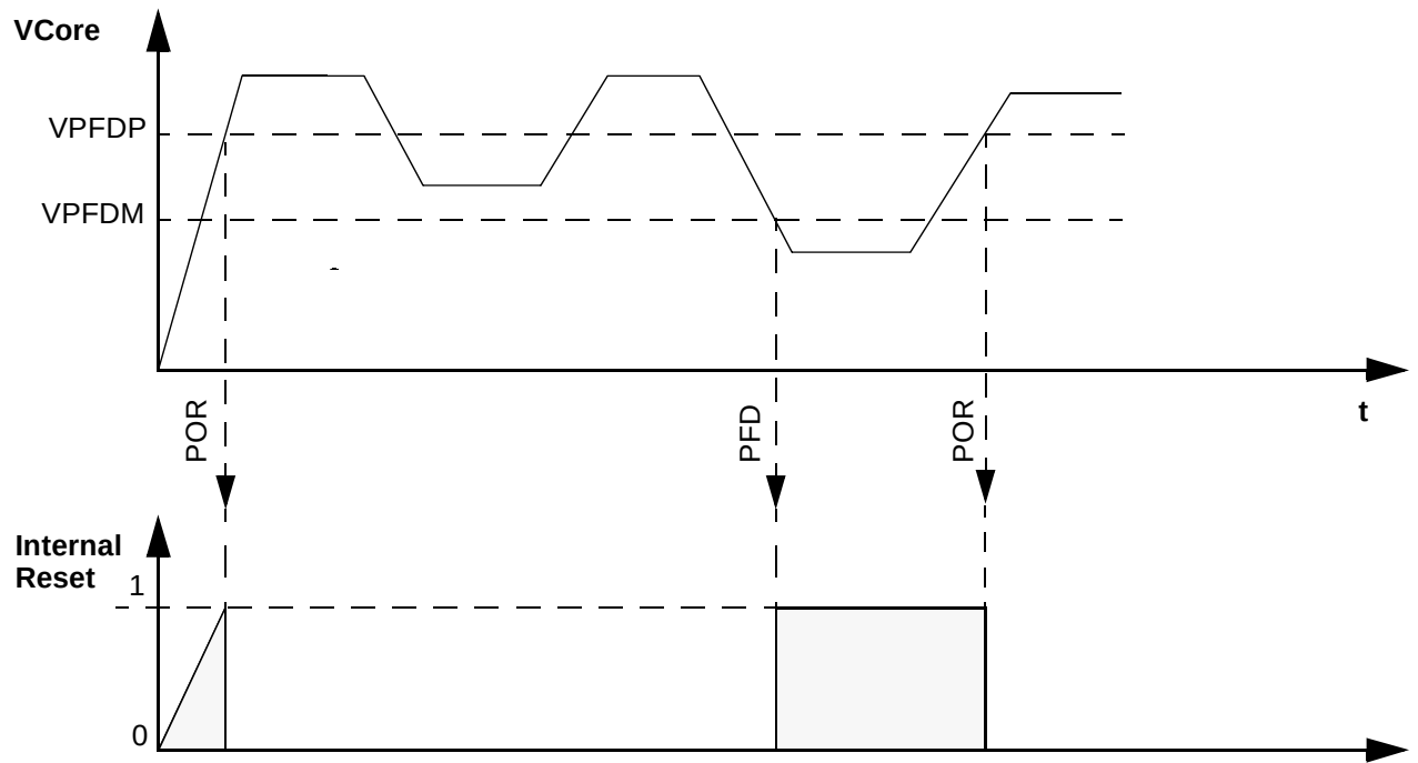
Figure 102. Static behaviour of POR and PFD
