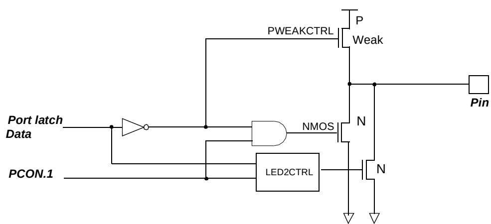
Figure 28. Low-speed Output
