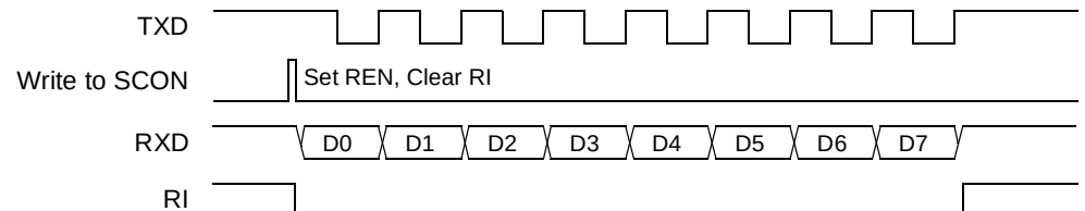
Figure 72. Reception Waveforms (Mode 0)
