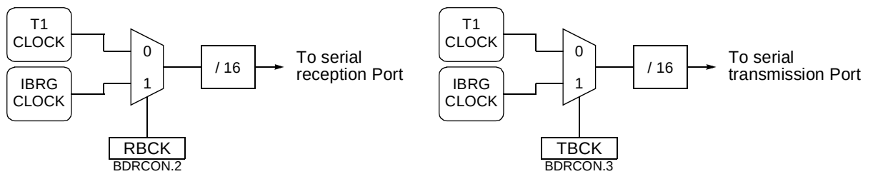
Figure 80. Baud Rate Formulas (Modes 1 and 3)
