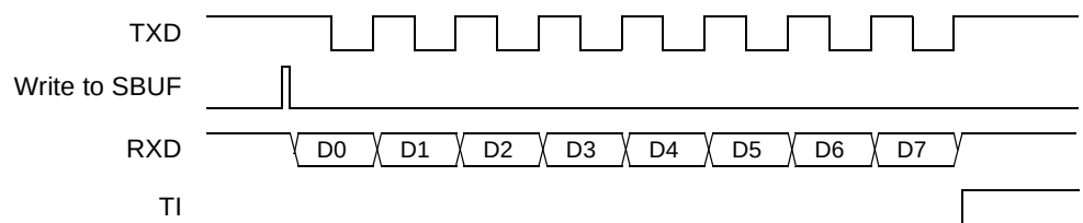
Figure 71. Transmission Waveforms (Mode 0)
