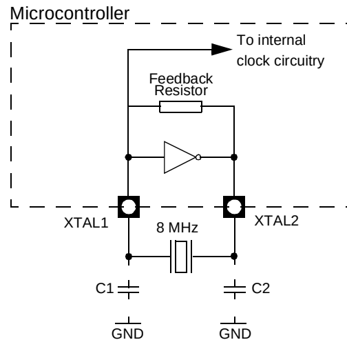
Figure 16. Oscillator Schematic
