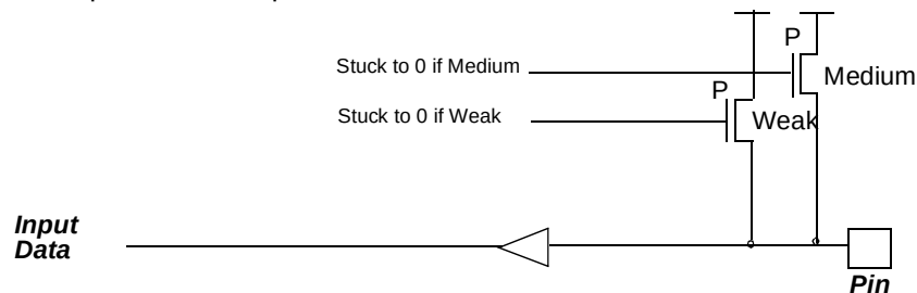
Figure 26. Input with Pull-up
