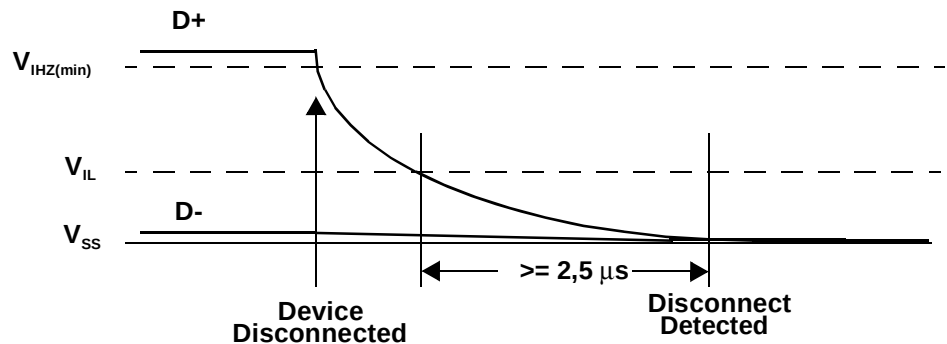
Figure 62. Disconnect Timing
