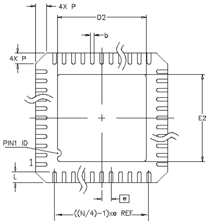
BOTTOM VIEW
