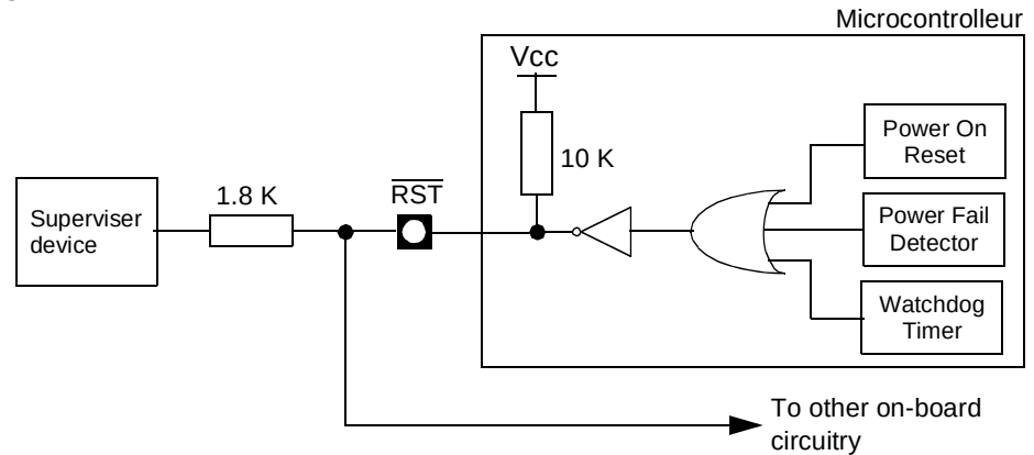
Figure 106. Use of an External Serial Resistor
