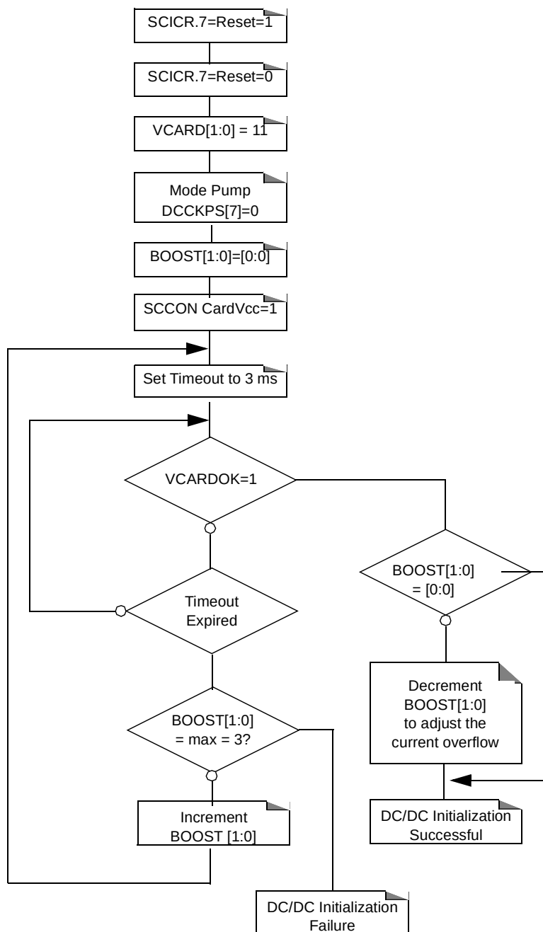
Figure 48. Card Vcc = 5V Initialization Procedure
