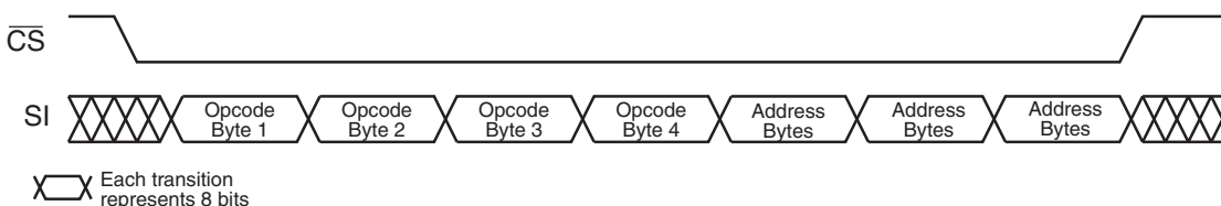
Figure 8-1. Sector Lockdown
