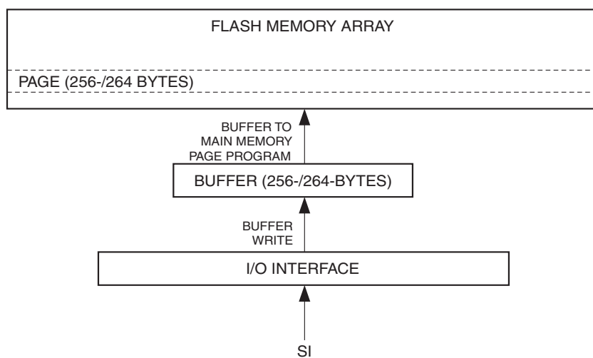
Figure 17-9. Write Operations
