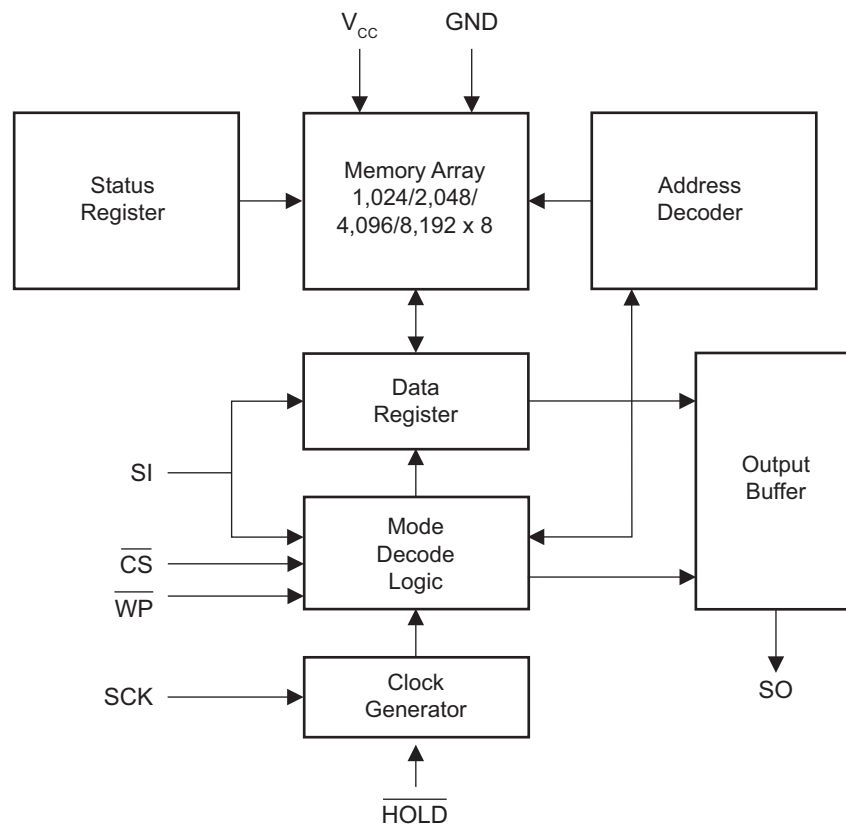
Figure 3-1. Block Diagram
