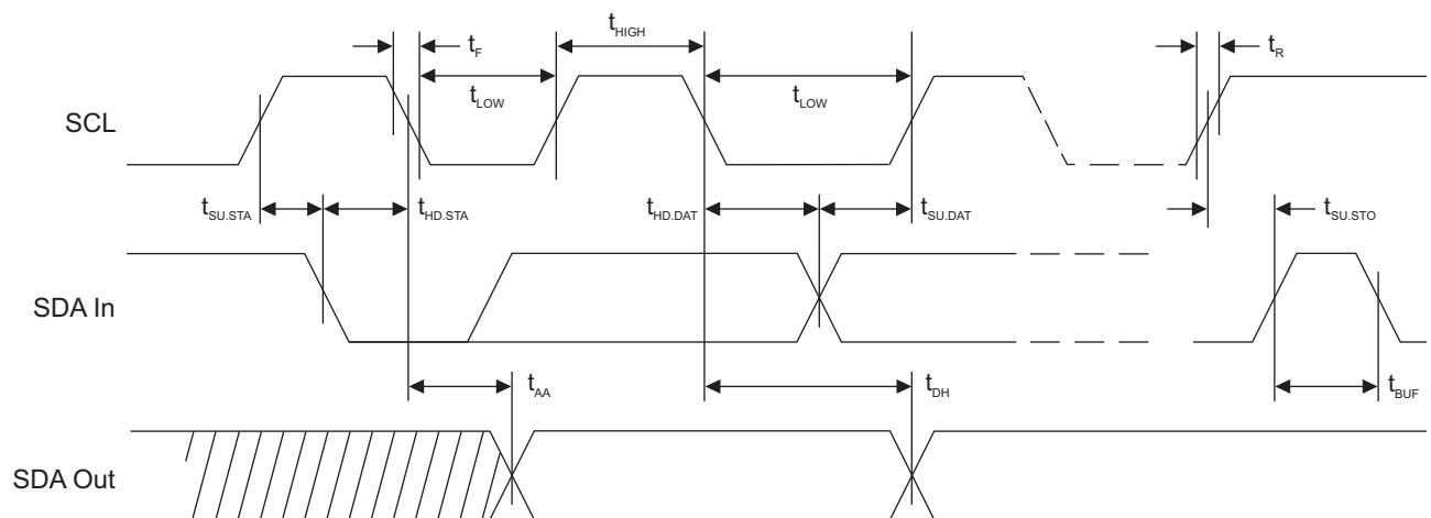
Figure 6-5. Bus Timing
