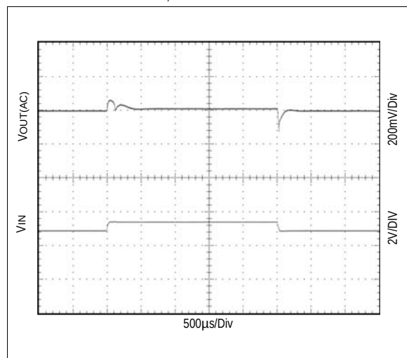
Figure 22. Transient Line Regulation; V_{OUT} = 18V , I_{LOAD} = 20mA
