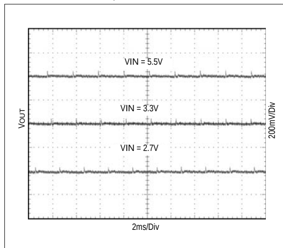
Figure 24. Output Voltage Ripple; V_{OUT} = 18V , I_{OUT} = 20mA
