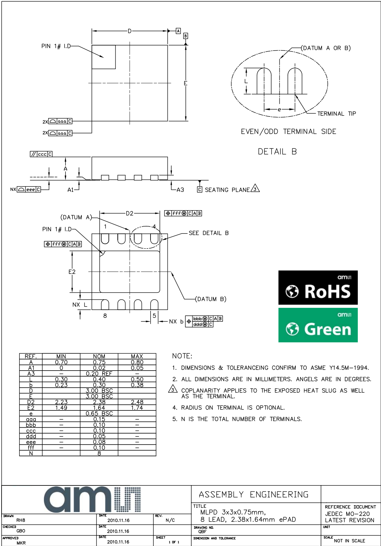
Figure 33. TDFN-8 3x3mm Package
