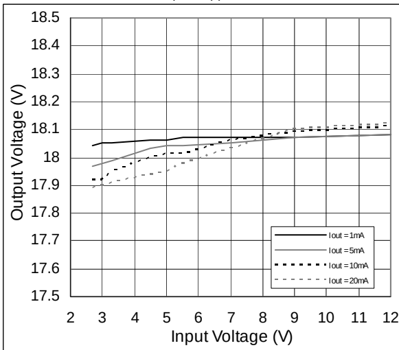
Figure 11. Output Voltage vs. Input Voltage; V_{OUT} = 18V , Split Supplies
