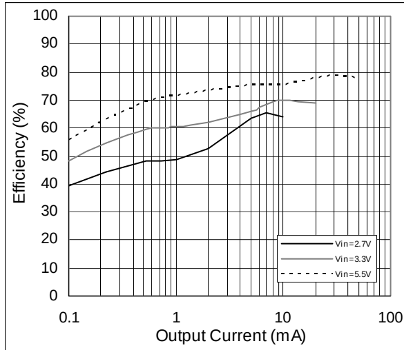
Figure 5. Efficiency vs. Output Current; V OUT = 12V
