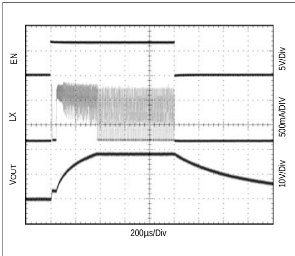
Figure 19. Startup Waveform
