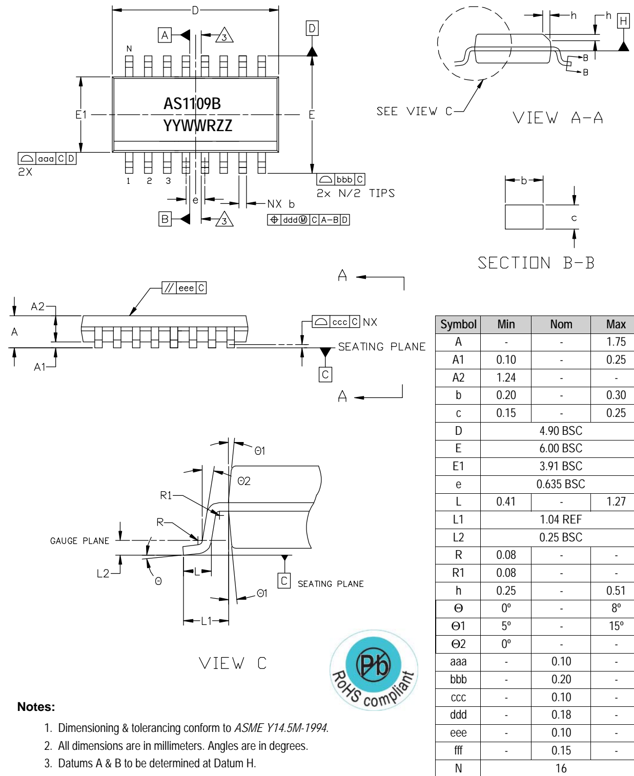
Figure 26. 16-pin QSOP-150 Package
