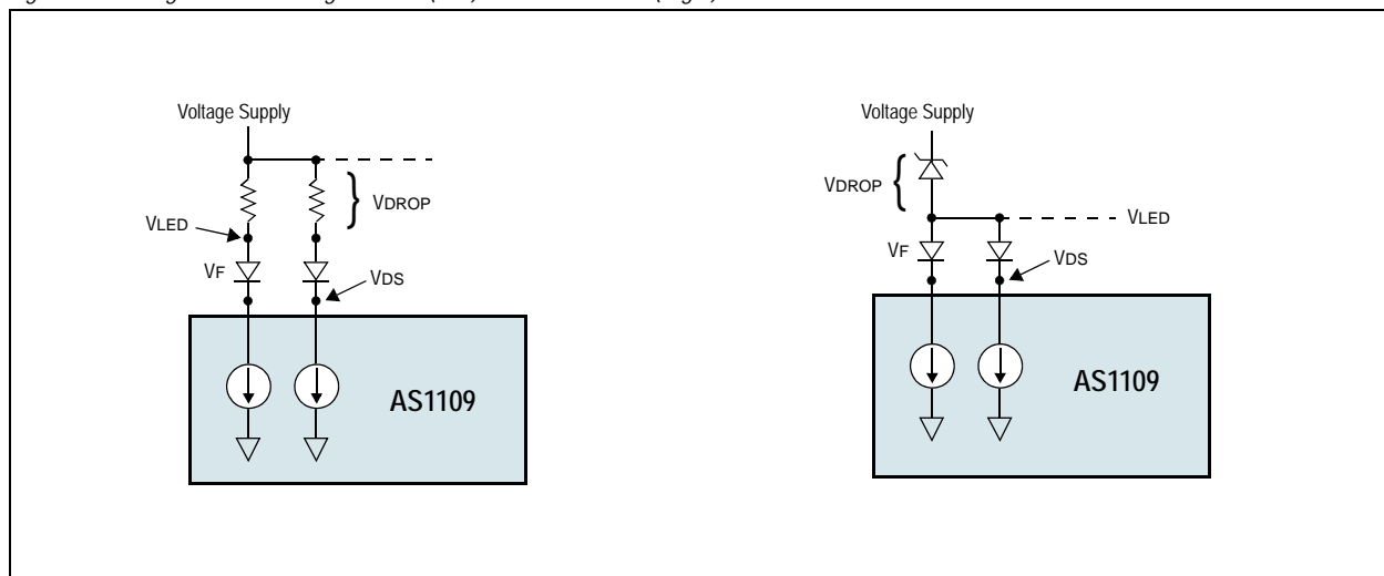
Figure 24. Voltage Reducer using Resistor (Left) and Zener Diode (Right)
