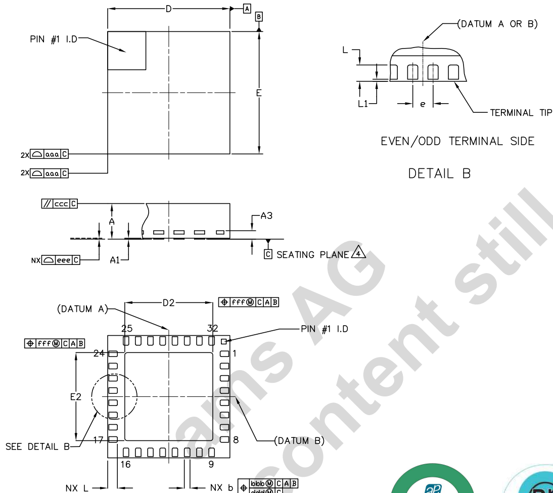
Figure 20. 32-pin TQFN 5x5 mm Package
