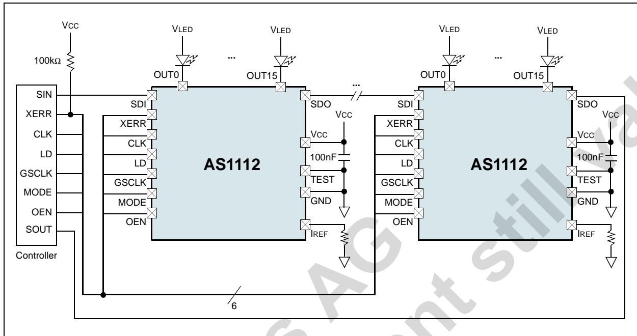
Figure 17. Cascaded Configuration
