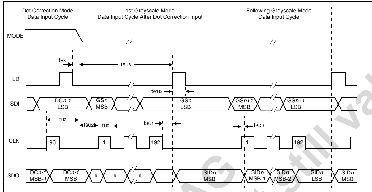
Figure 14. Greyscale Data Input Timing Diagram
