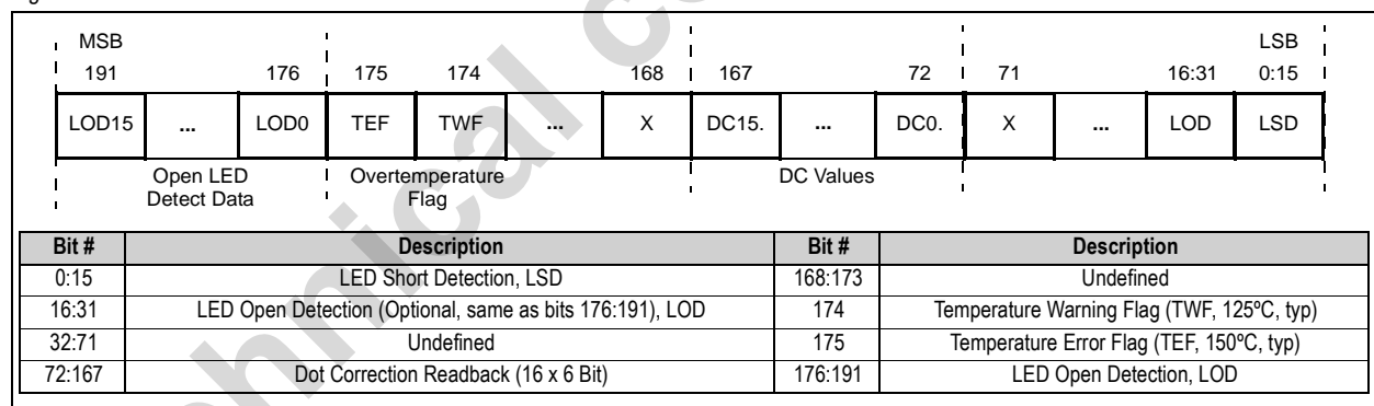
Figure 15. Status Information Data Packet Format
