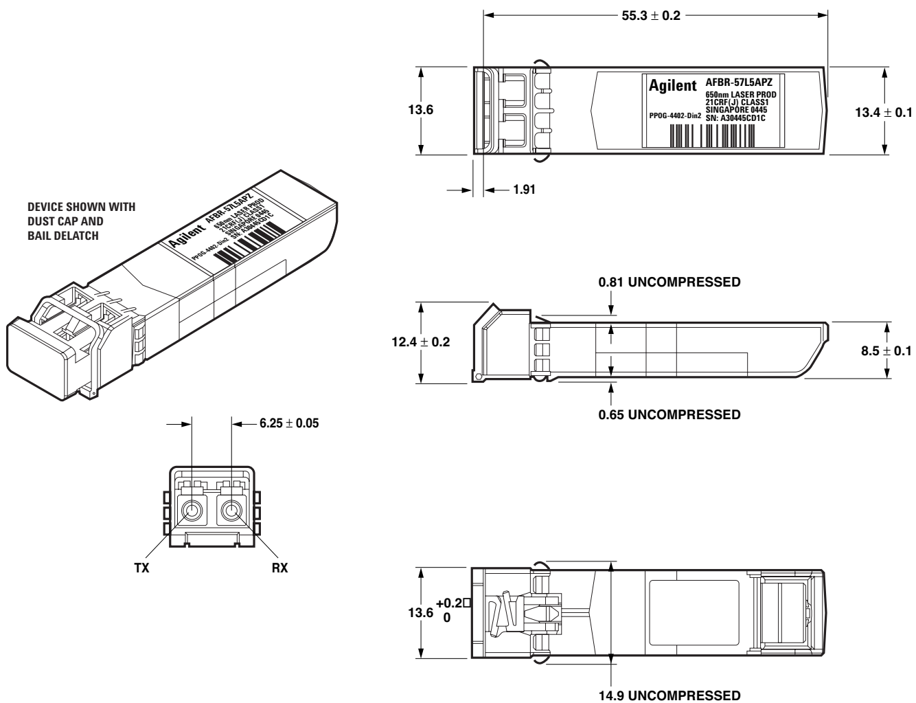
Figure 5. Module drawing.
