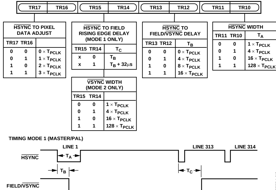
Figure 44. Timing Register 1
