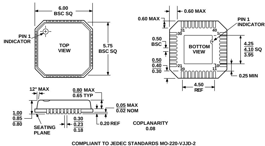
Figure 81. 40-Lead Lead Frame Chip Scale Package [LFCSP_VQ] 6 mm × 6 mm Body, Very Thin Quad (CP-40-1) Dimensions shown in millimeters
