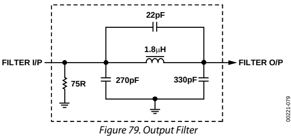
Figure 79. Output Filter
