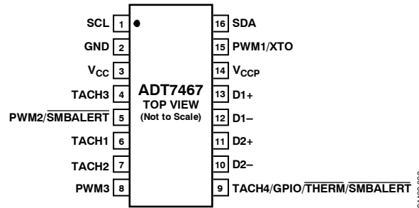
Figure 3. Pin Configuration
