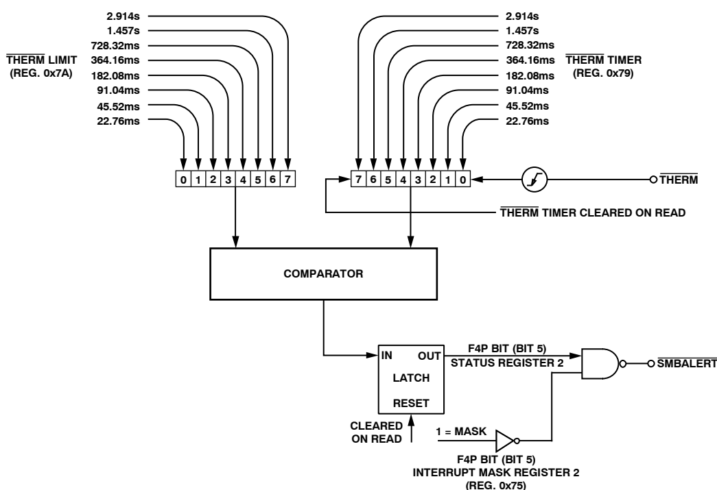
Figure 32. Functional Block Diagram of THERM Monitoring Circuitry
