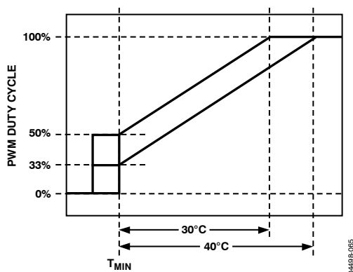
Figure 62. Adjusting \text{PWM}_{\text{MIN}} Affects T_{\text{RANGE}}
