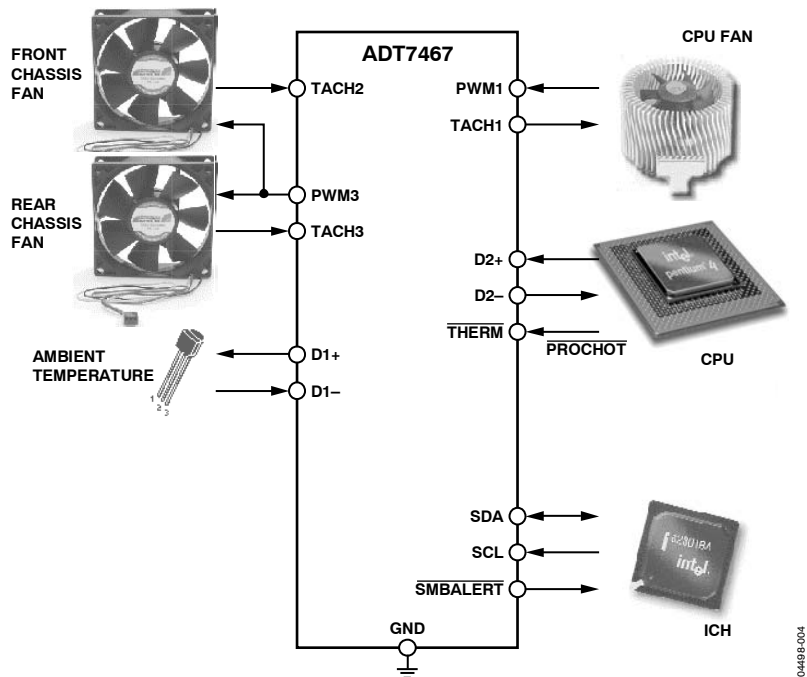
Figure 15. ADT7467 Configuration
