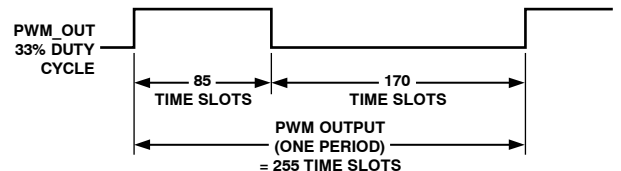
Figure 82. 33% PWM Duty Cycle, Represented in Time Slots
