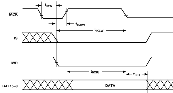
Figure 23. IDMA Write, Long Write Cycle
