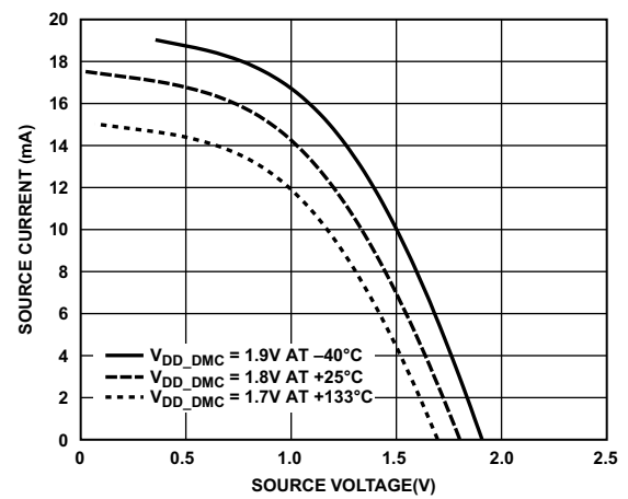
Figure 92. Driver Type B and Driver Type C (DDR2 Drive Strength 60 \Omega )
