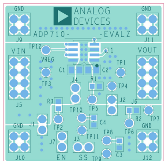
Figure 79. Example SOIC PCB Layout
