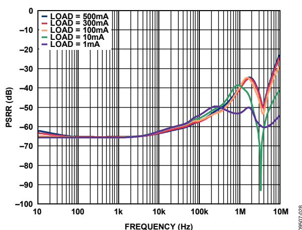
Figure 33. Power Supply Rejection Ratio vs. Frequency, V_{OUT} = 1.8\text{ V} , V_{IN} = 3.3\text{ V}
