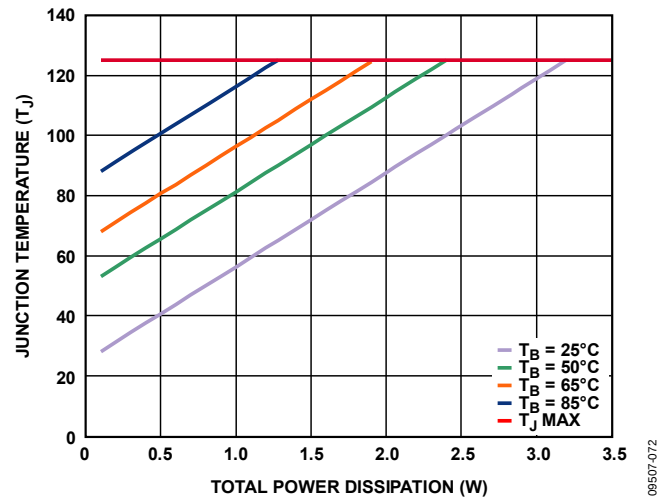
Figure 77. SOIC
