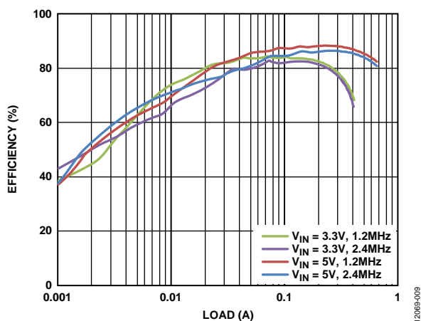
Figure 10. Boost Regulator Efficiency vs. Current Load, V_{POS} = 9\text{ V} , T_A = 25^\circ\text{C}
