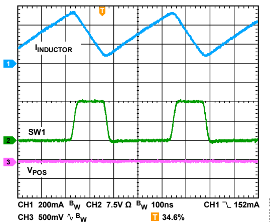
Figure 36. Boost Regulator Continuous Conduction Mode Operation Showing Inductor Current ( I_{INDUTOR} ), Switch Node Voltage, and Output Ripple, V_{IN} = 5\text{ V} , V_{POS} = 15\text{ V} , I_{LOAD1} = 90\text{ mA} , f_{SW} = 2.4\text{ MHz} , T_A = 25^\circ\text{C}
