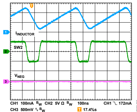
Figure 39. Inverting Regulator Continuous Conduction Mode Operation Showing Inductor Current ( I_{INDUTOR} ), Switch Node Voltage, and Output Ripple, V_{IN} = 5\text{ V} , V_{NEG} = -5\text{ V} , I_{LOAD2} = 35\text{ mA} , f_{SW} = 2.4\text{ MHz} , T_A = 25^\circ\text{C}
