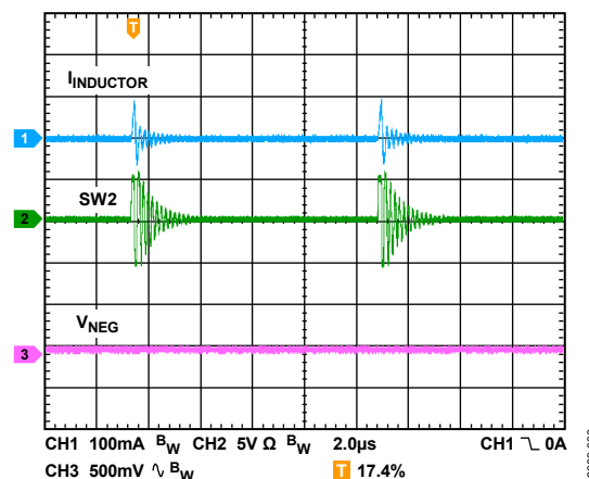
Figure 37. Inverting Regulator Skip Mode Operation Showing Inductor Current ( I_{INDUTOR} ), Switch Node Voltage, and Output Ripple, V_{IN} = 5\text{ V} , V_{NEG} = -5\text{ V} , I_{LOAD2} = 1\text{ mA} , f_{SW} = 2.4\text{ MHz} , T_A = 25^\circ\text{C}
