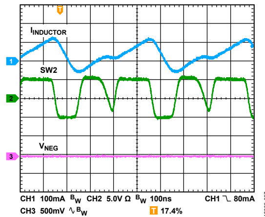
Figure 38. Inverting Regulator Discontinuous Conduction Mode Operation Showing Inductor Current ( I_{INDUTOR} ), Switch Node Voltage, and Output Ripple, V_{IN} = 5\text{ V} , V_{NEG} = -5\text{ V} , I_{LOAD2} = 6\text{ mA} , f_{SW} = 2.4\text{ MHz} , T_A = 25^\circ\text{C}
