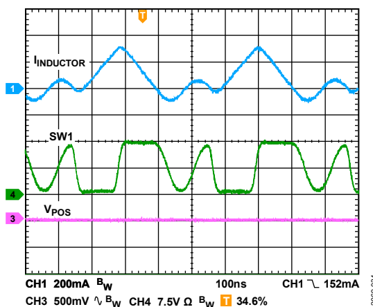
Figure 35. Boost Regulator Discontinuous Conduction Mode Operation Showing Inductor Current ( I_{INDUTOR} ), Switch Node Voltage, and Output Ripple, V_{IN} = 5\text{ V} , V_{POS} = 15\text{ V} , I_{LOAD1} = 20\text{ mA} , f_{SW} = 2.4\text{ MHz} , T_A = 25^\circ\text{C}
