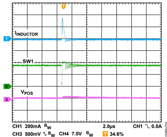
Figure 34. Boost Regulator Skip Mode Operation Showing Inductor Current ( I_{INDUTOR} ), Switch Node Voltage, and Output Ripple, V_{IN} = 12\text{ V} , V_{POS} = 15\text{ V} , I_{LOAD1} = 4\text{ mA} , f_{SW} = 2.4\text{ MHz} , T_A = 25^\circ\text{C}
