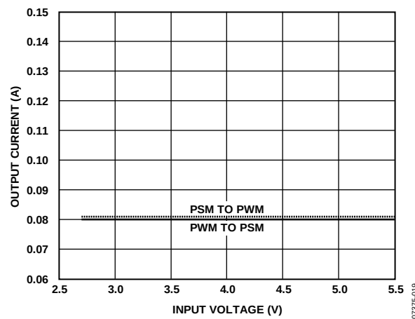
Figure 9. Mode Transition
