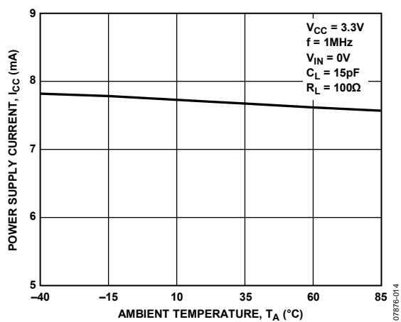
Figure 14. Power Supply Current vs. Ambient Temperature
