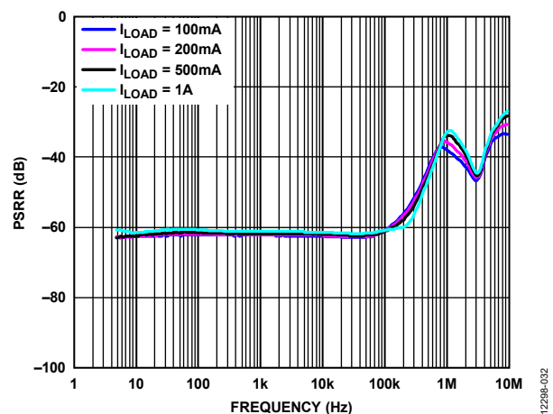
Figure 32. Power Supply Rejection Ratio (PSRR) vs. Frequency, 800\text{ mV} Headroom, V_{OUT} = 3\text{ V}
