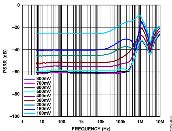
Figure 30. Power Supply Rejection Ratio (PSRR) vs. Frequency, V_{OUT} = 3\text{ V} , 1\text{ A} Load Current, Various Headroom Voltages
