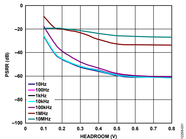
Figure 31. Power Supply Rejection Ratio (PSRR) vs. Headroom, V_{OUT} = 3\text{ V} , 1\text{ A} Load Current, Different Frequencies
