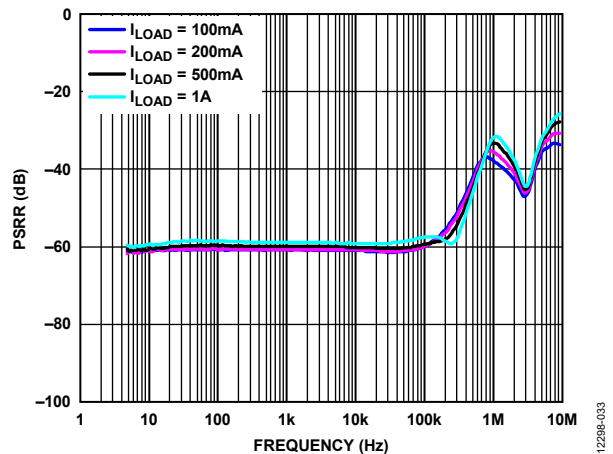
Figure 33. Power Supply Rejection Ratio (PSRR) vs. Frequency, 500\text{ mV} Headroom, V_{OUT} = 3\text{ V}
