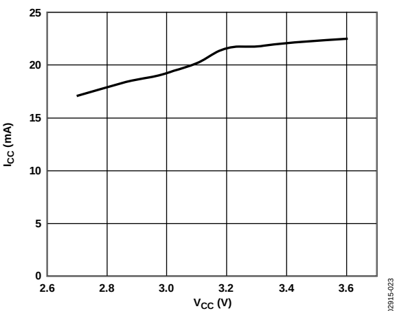
Figure 23. I_{CC} vs. V_{CC} ( R_L = 3\text{ k}\Omega )
