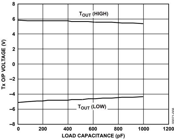
Figure 8. Transmitter Output Voltage High/Low vs. Load Capacitance @ 460 kbps
