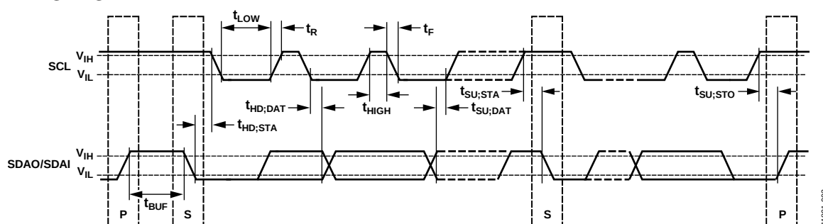
Figure 3. Serial Bus Timing Diagram
