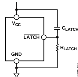
Figure 23. \overline{\text{LATCH}} Pin Delay Circuit
