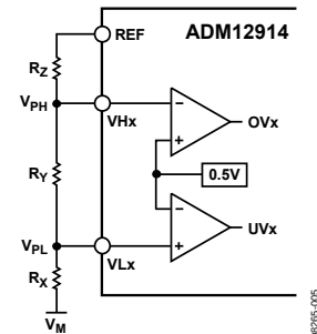
Figure 18. Negative Undervoltage/Overvoltage Monitoring Configuration
