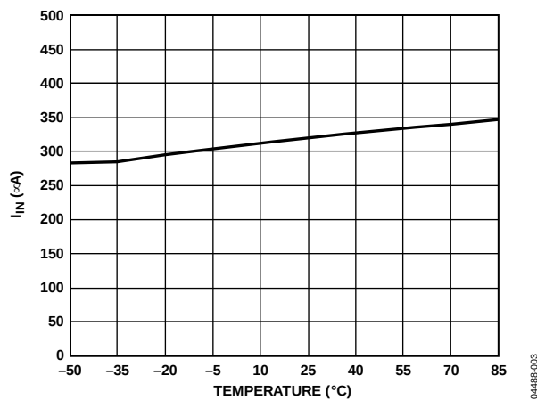
Figure 3. I_{IN} vs. Temperature
