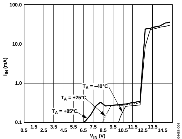
Figure 4. I_{IN} vs. V_{IN}
