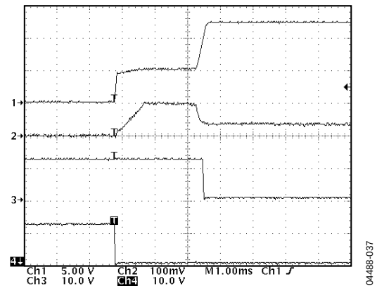
Figure 37. Typical Startup Sequence (Ch1 = GATE; Ch2 = SENSE; Ch3 = PWRGD; Ch4 = SPLYGD)
