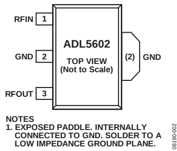
Figure 2. Pin Configuration
