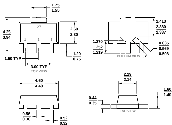
Figure 21. 3-Lead Small Outline Transistor Package [SOT-89]
