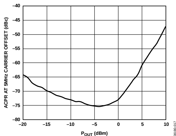
Figure 18. ACPR vs. P_{OUT} , Single Carrier W-CDMA (Test Model 1-64) at 2140 MHz Evaluation Board
