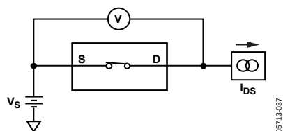
Figure 31. On Resistance
