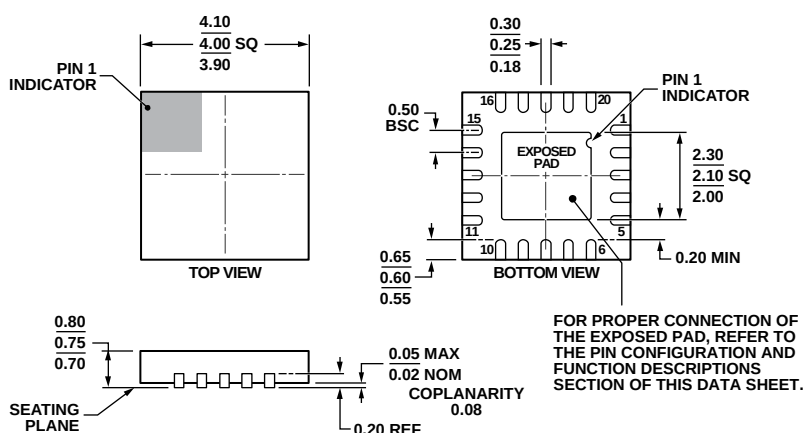
Figure 25. 20-Lead Lead Frame Chip Scale Package [LFCSP] 4 mm x 4 mm Body, and 0.75 mm Package Height (CP-20-6)
