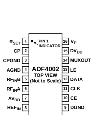
Figure 3. TSSOP Pin Configuration (Top View)
