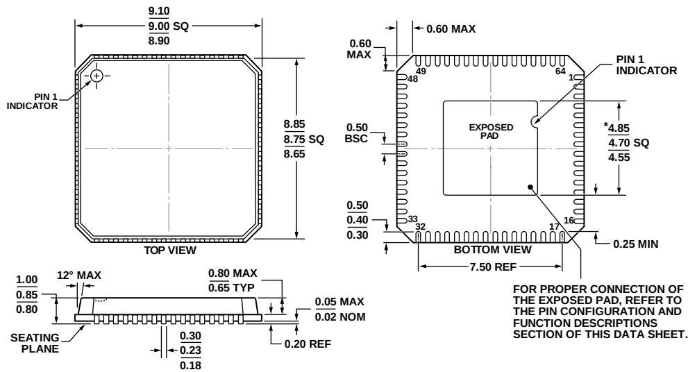
*COMPLIANT TO JEDEC STANDARDS MO-220-VMM-D-4 EXCEPT FOR EXPOSED PAD DIMENSION Figure 6. 64-Lead Lead Frame Chip Scale Package [LFCSP_VQ] 9 mm × 9 mm Body, Very Thin Quad (CP-64-1) Dimensions shown in millimeters
