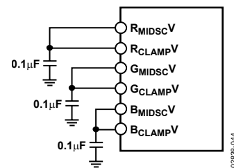
Figure 4. Typical Clamp Configuration for RGB and YUV Applications
