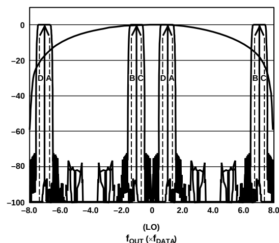
Figure 88. 8x Interpolation, Complex f_{DAC}/8 Modulation
