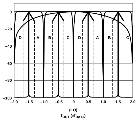
Figure 83. 2x Interpolation, Complex f_{DAC}/4 Modulation
