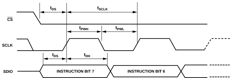
Figure 35. Timing Diagram for Register Write to AD9773
