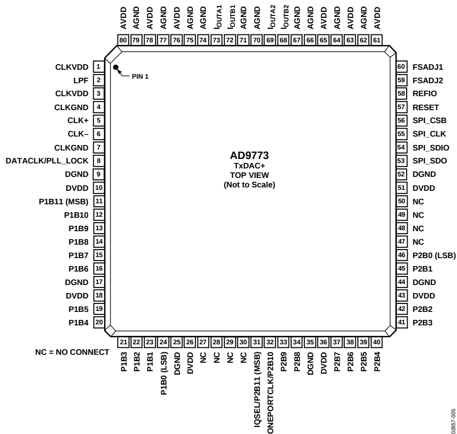
Figure 5. Pin Configuration
