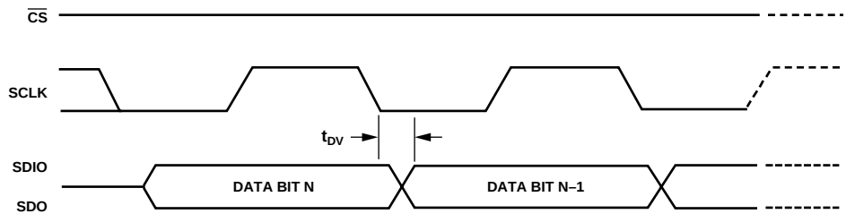
Figure 36. Timing Diagram for Register Read from AD9773
