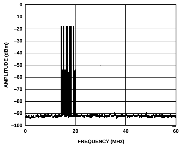
Figure 31. Eight-Tone IMD Performance, f_{DATA} = 160 MSPS, Interpolation = 8×
