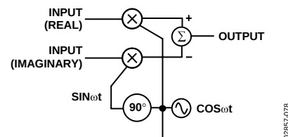
Figure 78. Quadrature Modulator
